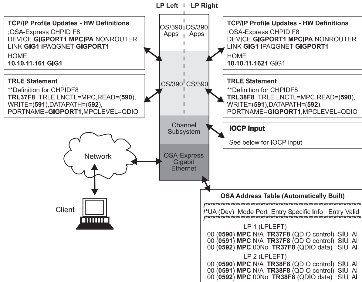
Figure E-12. OSA Configuration with Two Logical Partitions
