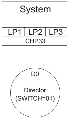
Figure E-5. FICON CTC and Director with Single Path
