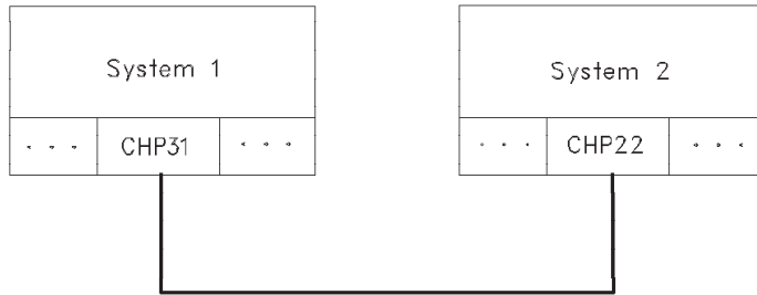
Figure E-3. ESCON CTC Point-to-Point
