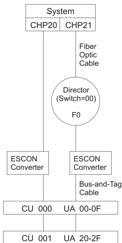
Figure E-9. Channels Through an ESCON Converter
