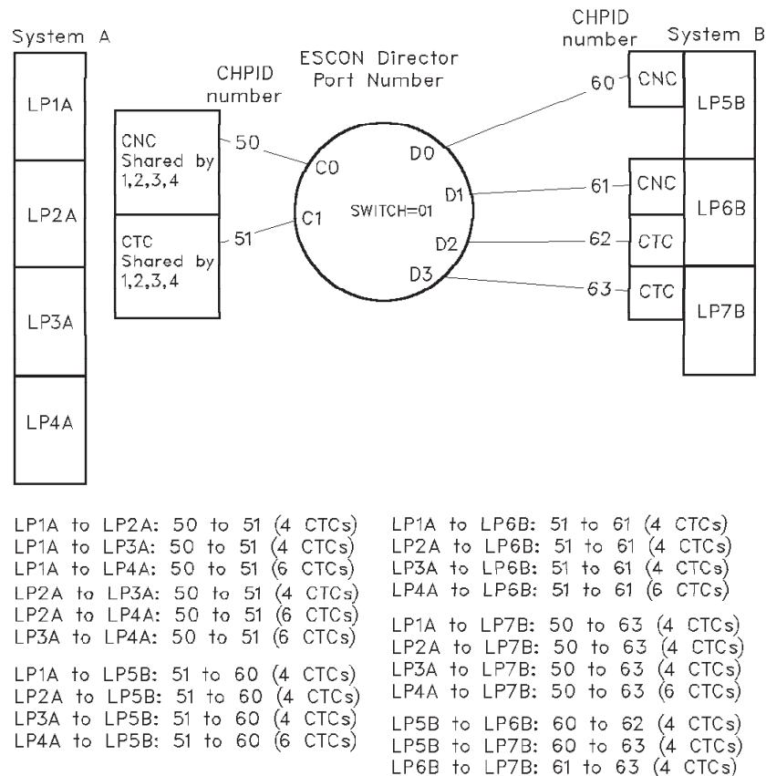
Figure E-16. ESCON CTC with Shared and Unshared Channels
