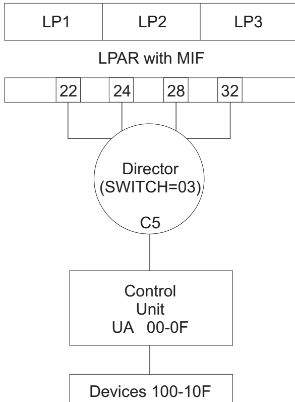
Figure E-2. LPAR Mode with Shared Paths to an ESCON Device
