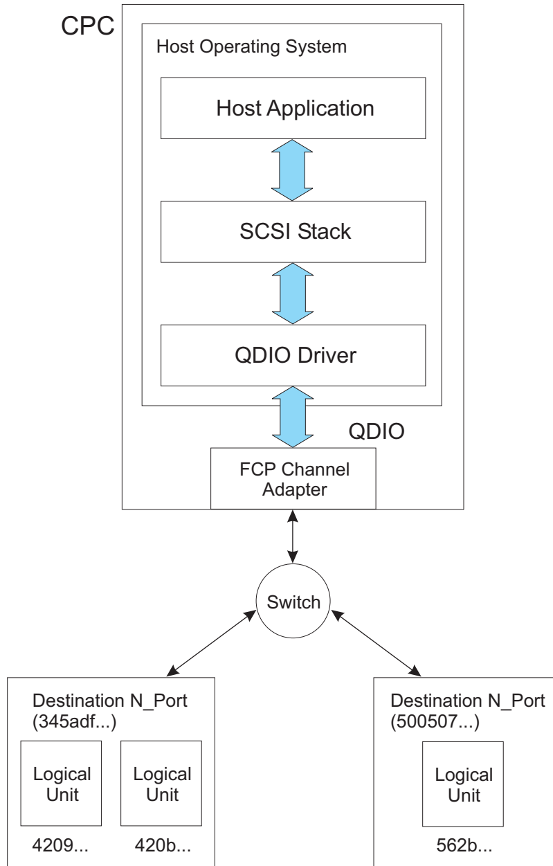
Figure E-14. FCP Channel Configuration
