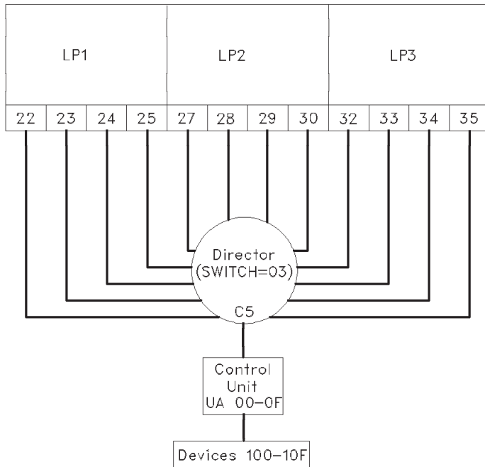
Figure E-1. LPAR Mode with More Than Eight Paths to an ESCON Device
