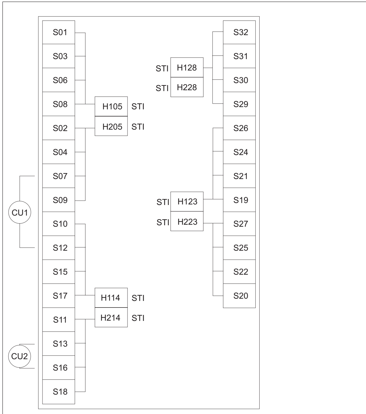
Figure 1-2. I/O Channel Path Configuration for a Representative I/O Cage in a 2094 or 2096 Model
