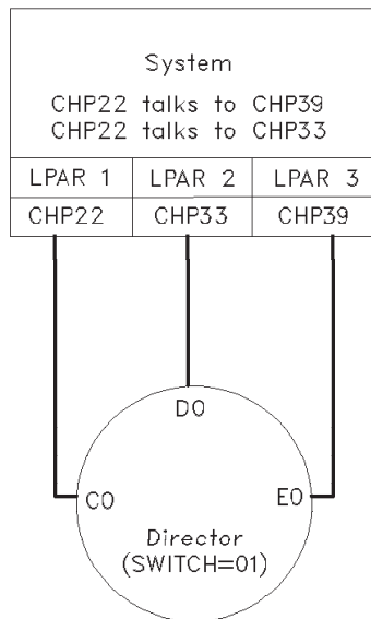
Figure E-4. ESCON CTC Dynamic Through an ESCON Director with Multiple Paths
