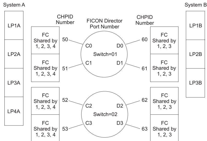
Figure E-18. FICON CTC (Fully Redundant)
