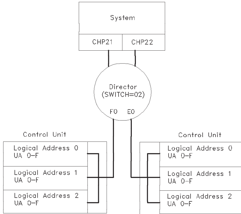
Figure E-8. Control Unit Logical Addressing
