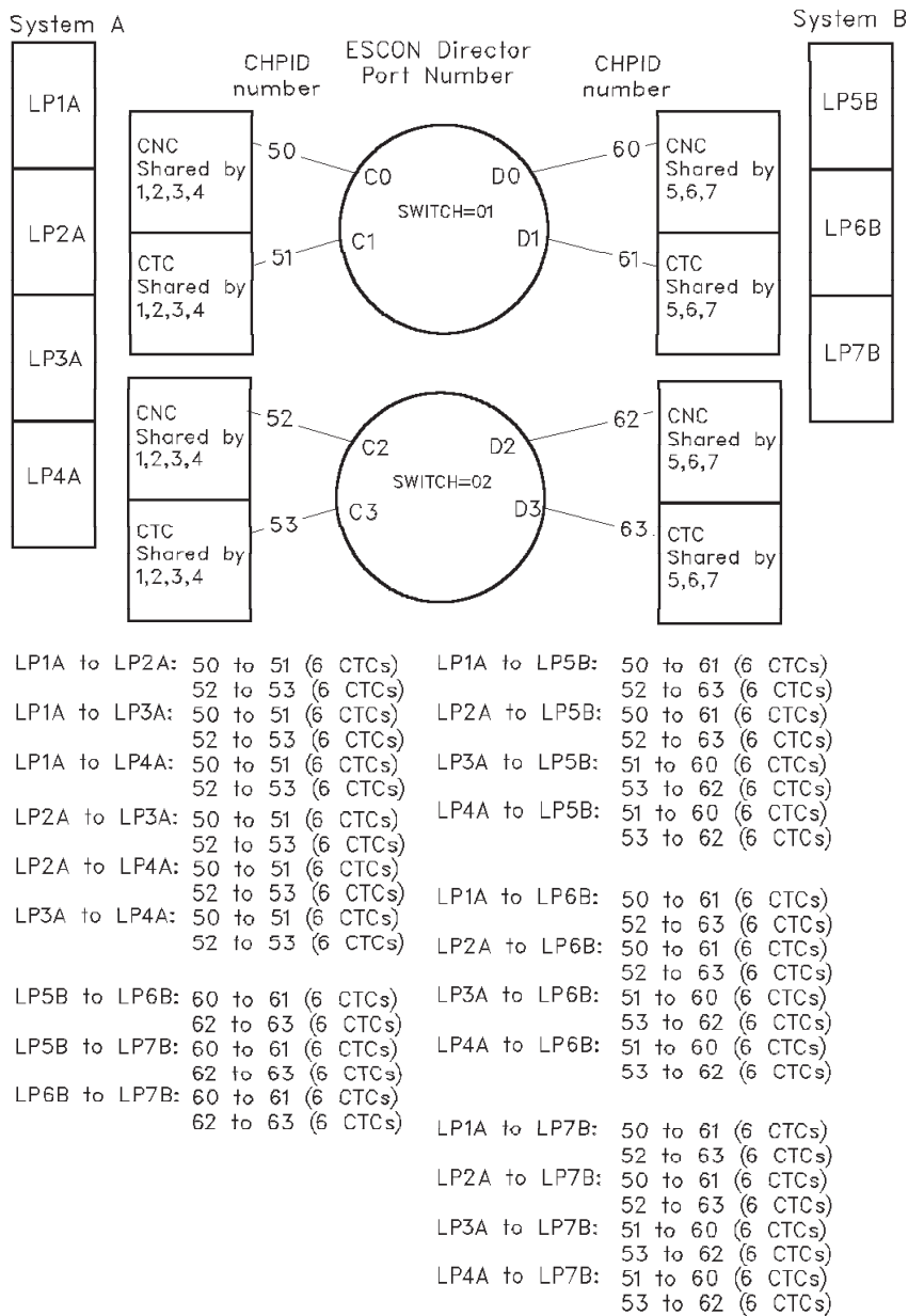
Figure E-17. ESCON CTC with Shared Channels
