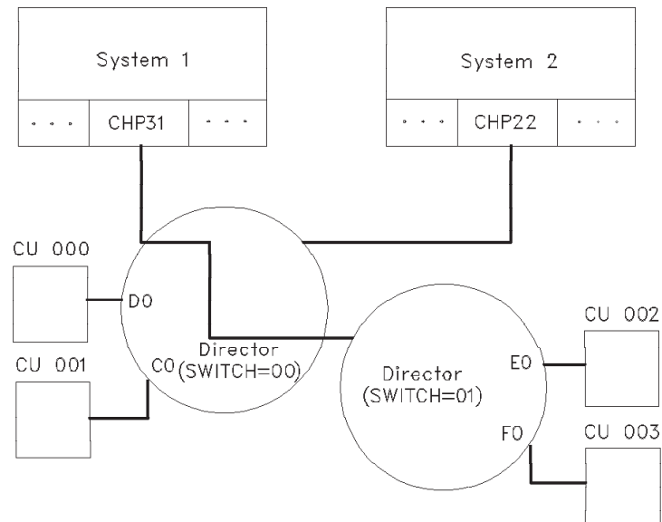
Figure E-6. Chained ESCON Directors
