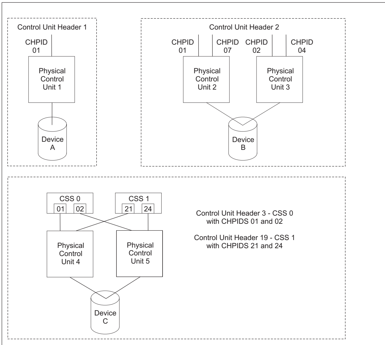
Figure 1-4. Valid Control Unit Headers
