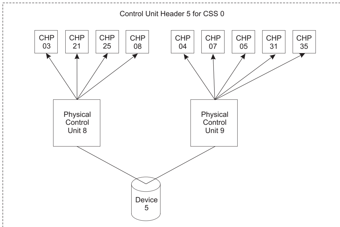
Figure 1-5. Control Unit Header That Is Incorrect
