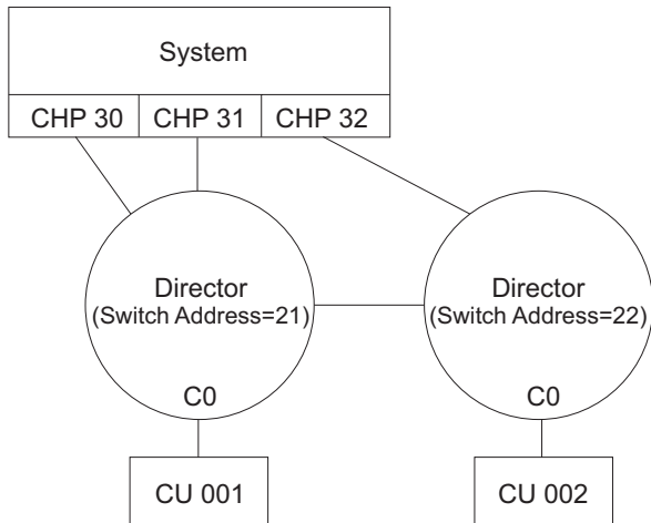
Figure E-7. Cascaded FICON Directors
